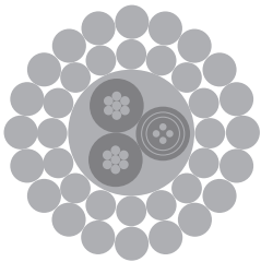
Electro-Optic Wireline
